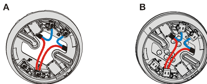
Figure 10: Detector base with screw terminals (A) and sockets (B)
