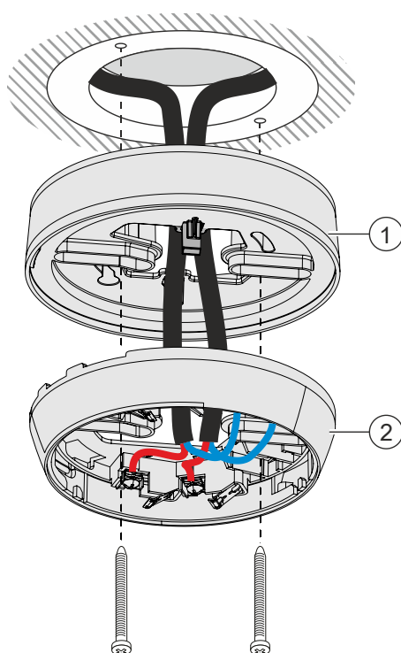
Figure 5: Recess-mounted cable entry with base attachment BA720
