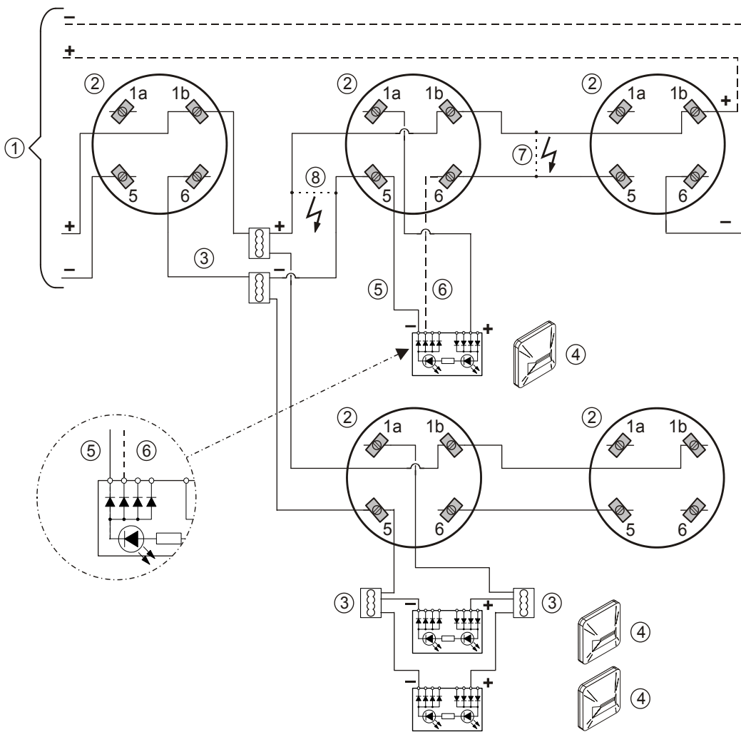
Figure 12: Connection diagram for addressed detector lines
